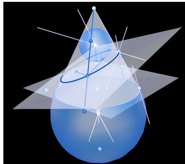
Figure 5: Proof of DANDELIN: A geometric proof that the intersection of plane and cone are either ellipse, hyperbola or parabola.
