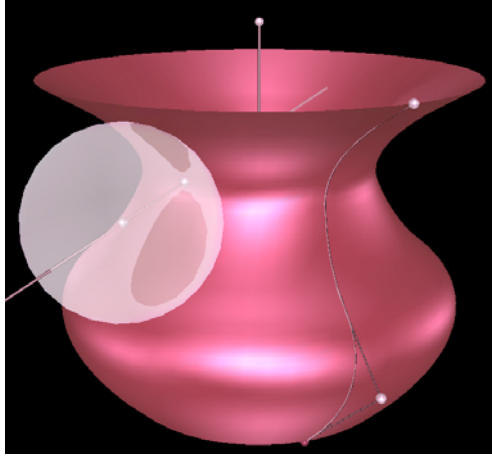
Figure 5: Milling of a surface of revolution. The milling head is a sphere.
