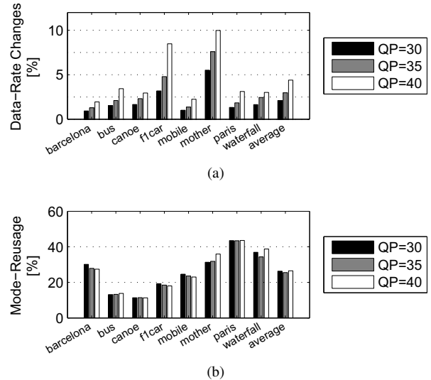
Figure 7. Average increase in the data-rate and mode-reusage using the single-criterion algorithm ( T = 10\% ). (a) The increases of the data-rate compared to the exhaustive Intra- 4 \times 4 mode-decision. (b) Percentage of 4 \times 4 -blocks with reused coding modes.
